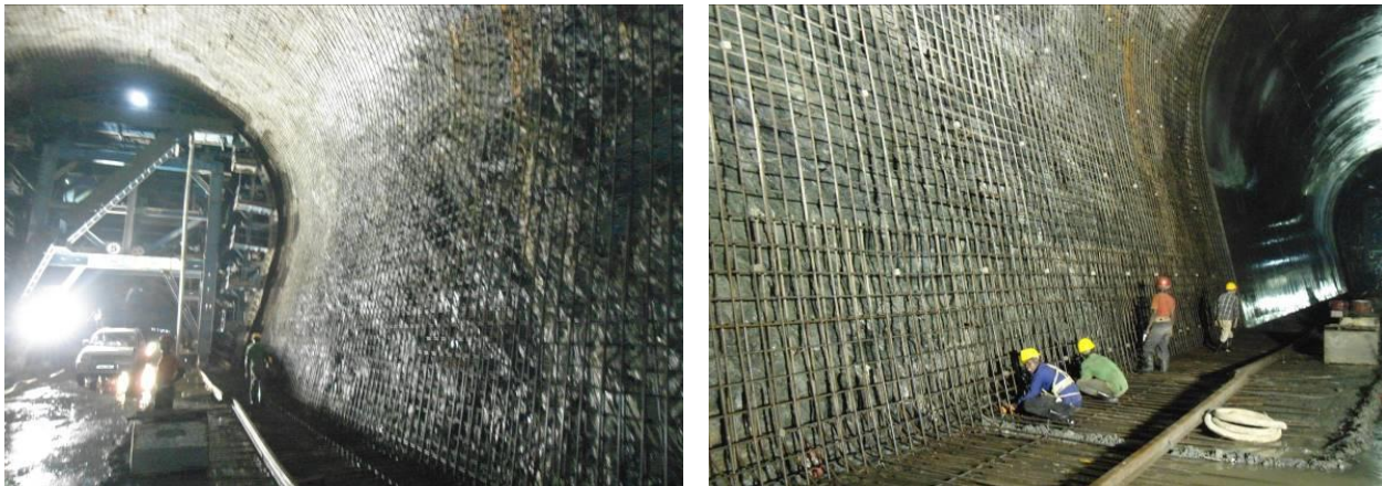
L-R: Completed excavations and ongoing steel works in preparation for concreting in the Tail Race Tunnel (TRT) at Karuma HPP in Nwoya/Kiryandongo district
